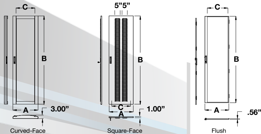
24" Width Curved-Face (Material: 18 GA. CRS)
