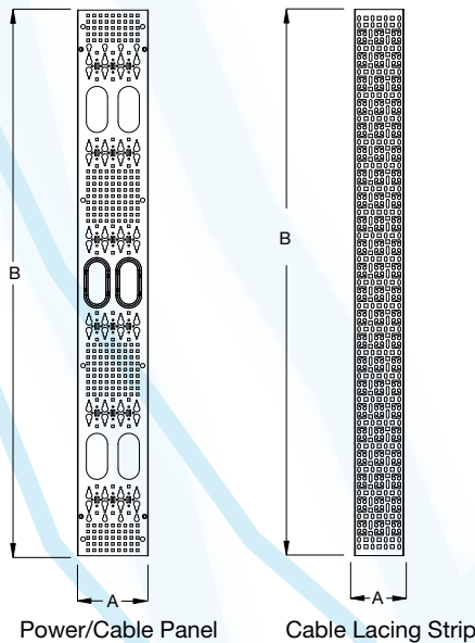
Power/Cable Panel (Material: 14 ga. CRS)
