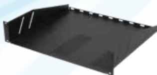
Vented Light Duty Shelf UA-SH1 (15 lb load rating) UA-SH2 (50 lb load rating) UA-SH3 (60 lb load rating) UA-SH4 (70 lb load rating) UA-SH5 (80 lb load rating)
