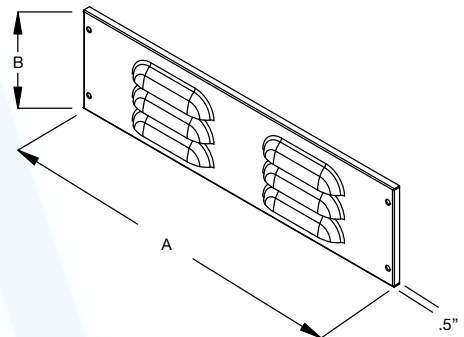
Louvered Enclosure Panel
