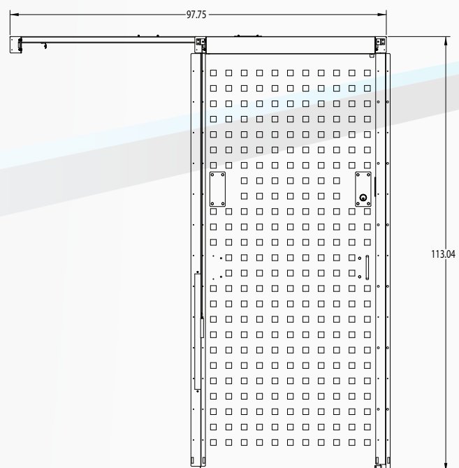
Perforated Sliding Door
