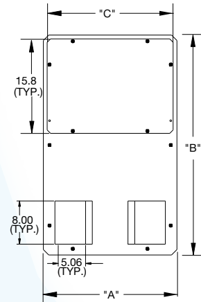
Cover Plate
