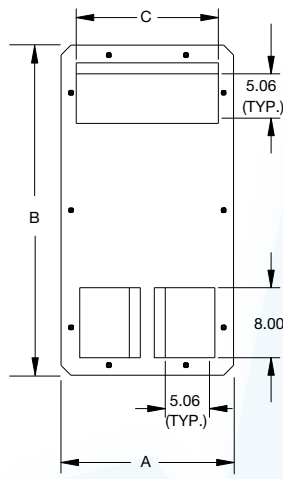
Brush Strip
